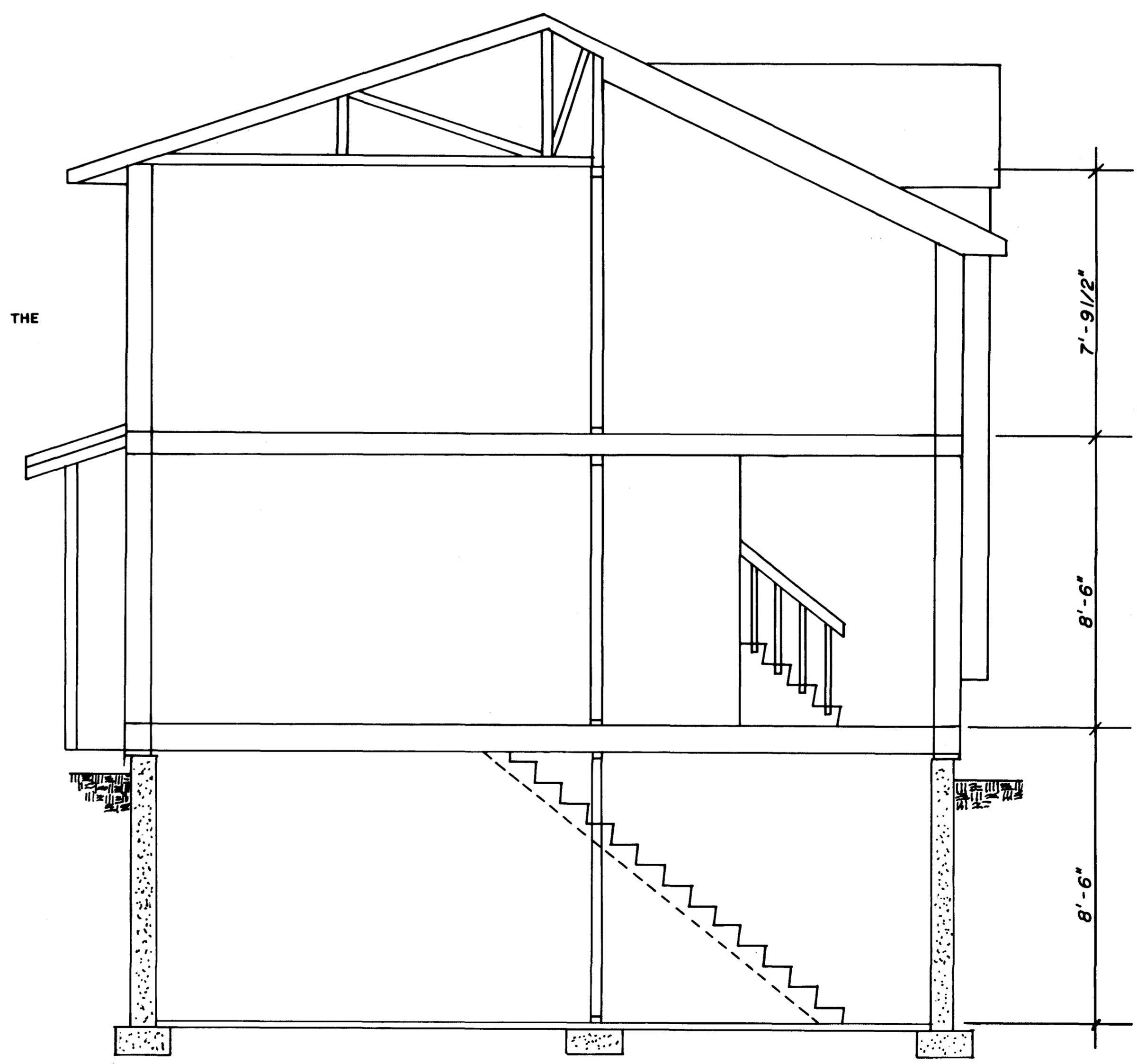
2 BEDROOM CROSS SECTION scale 3/8"=1'
