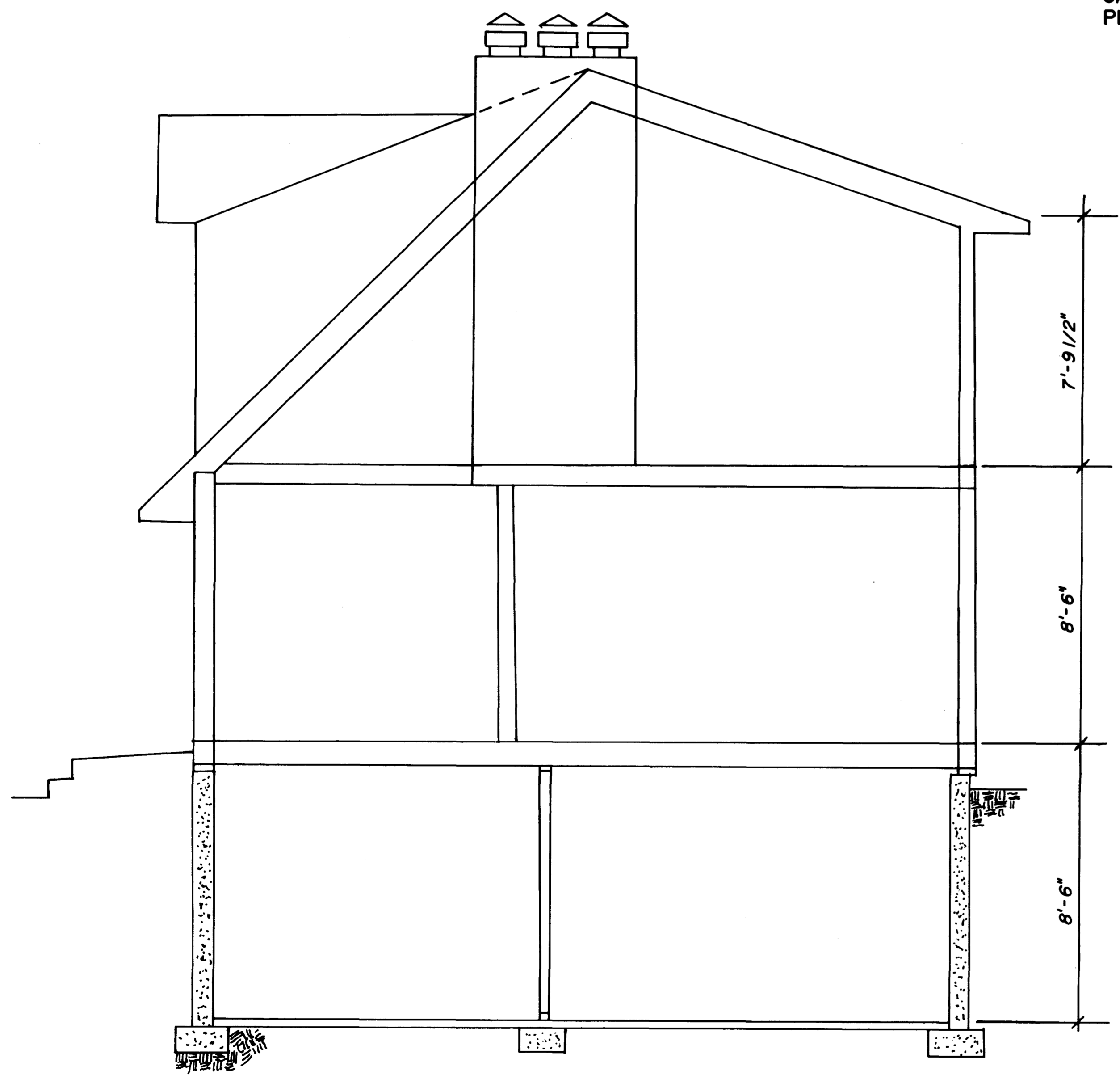
3 BEDROOM CROSS SECTION scale 3/8"=1'
